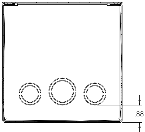
SECTION X-X
