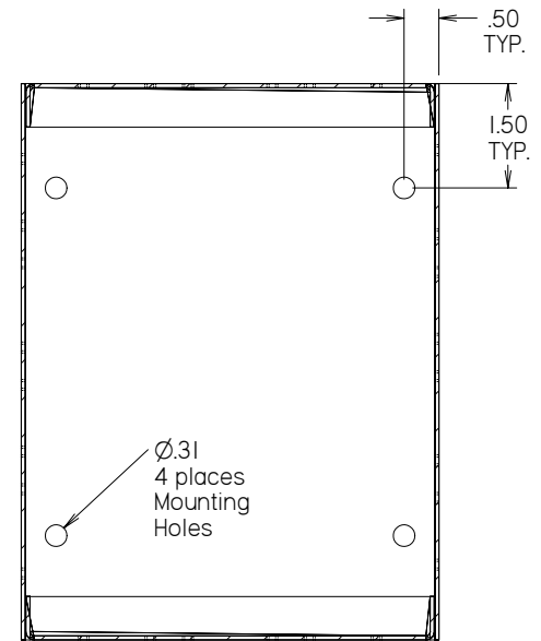
SECTION Y-Y
