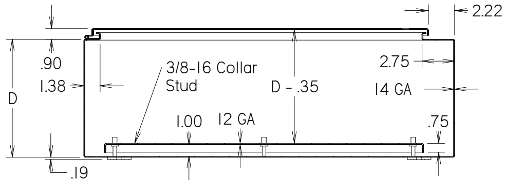
SECTION X-X
