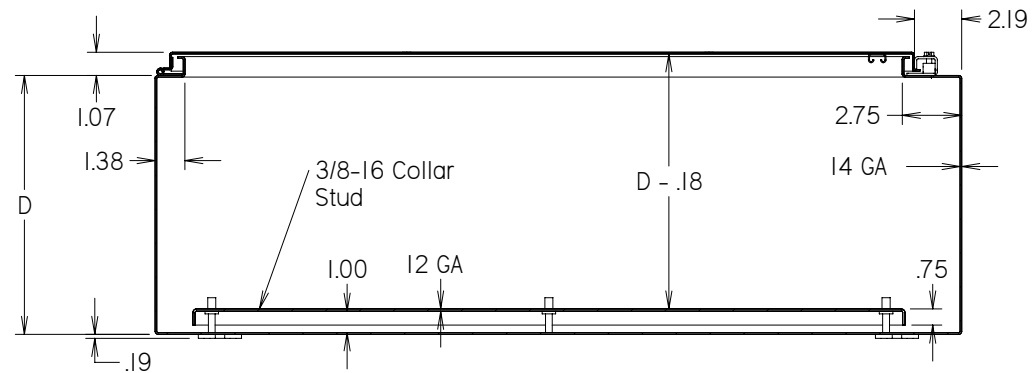
SECTION X-X
