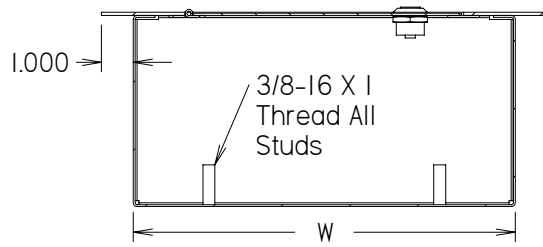
SECTION X-X
