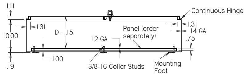
SECTION X-X
